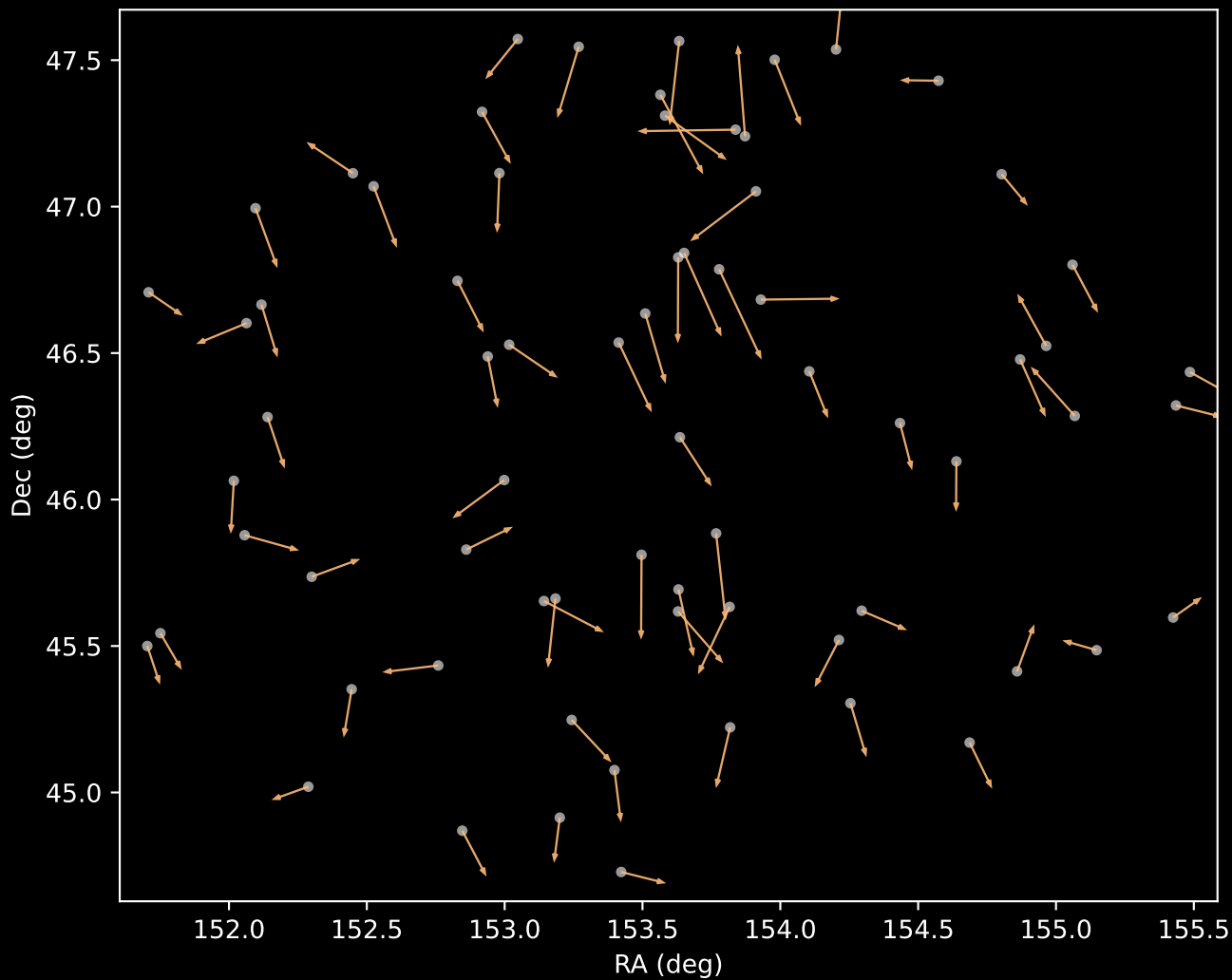
APOGEE DR17 Cluster 3 Proper Motion Vectors (n=70)
