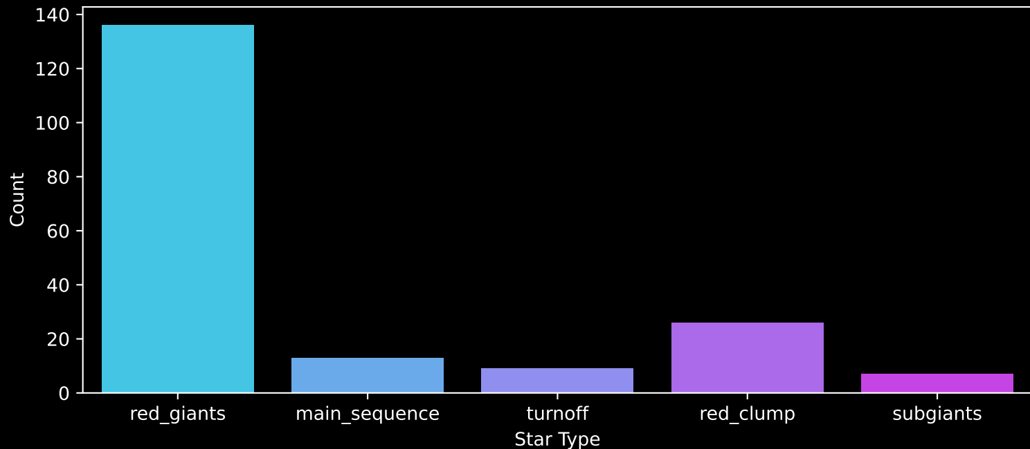
APOGEE DR17 Field: [150-08-RV] Count plot of Star Type
