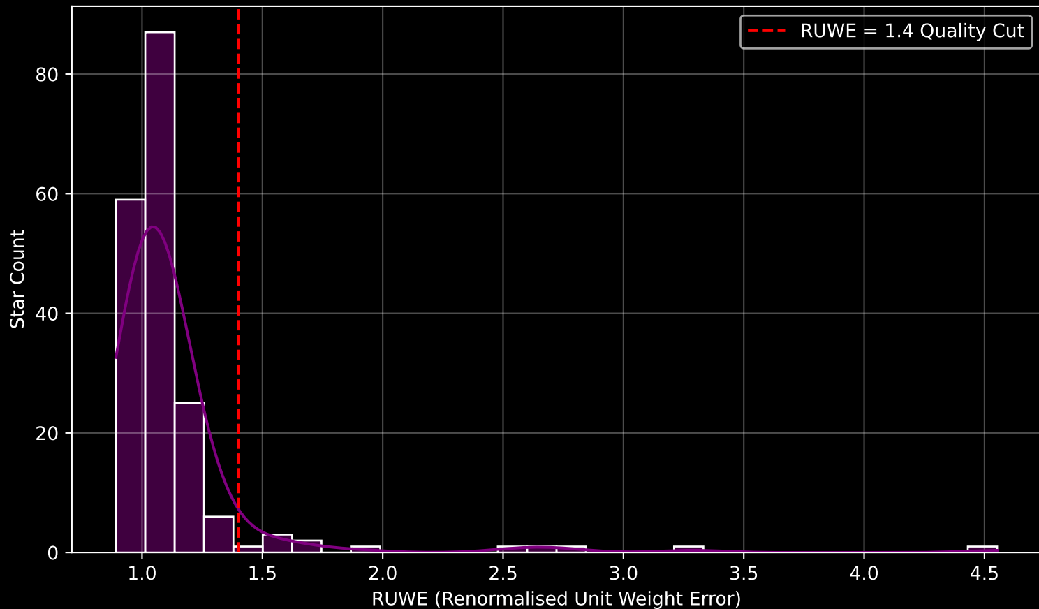
GAPOGEE DR17 Field [150-08-RV] RUWE Distribution (n= 189)
