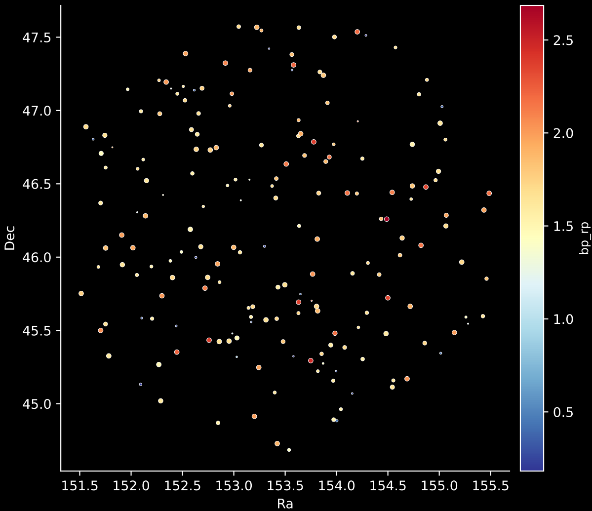
APOGEE DR17 Field: [150-08-RV] Stars: 191
