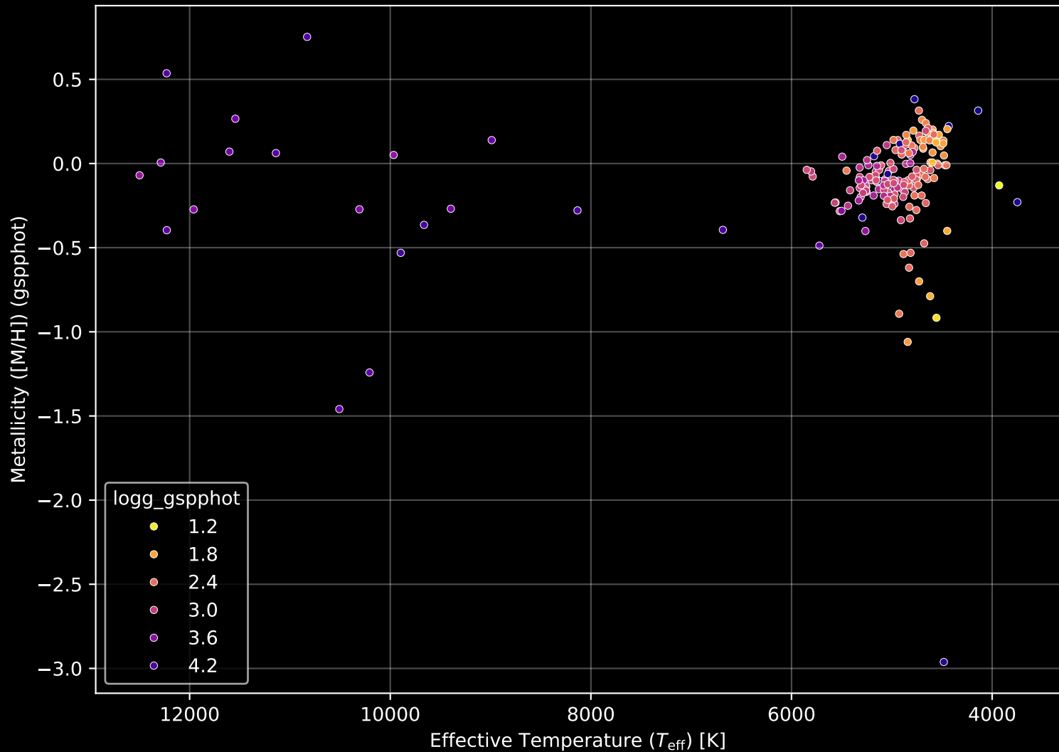
APOGEE DR17 Field: [150-08-RV] Stellar Population Parameters (n= 191)
