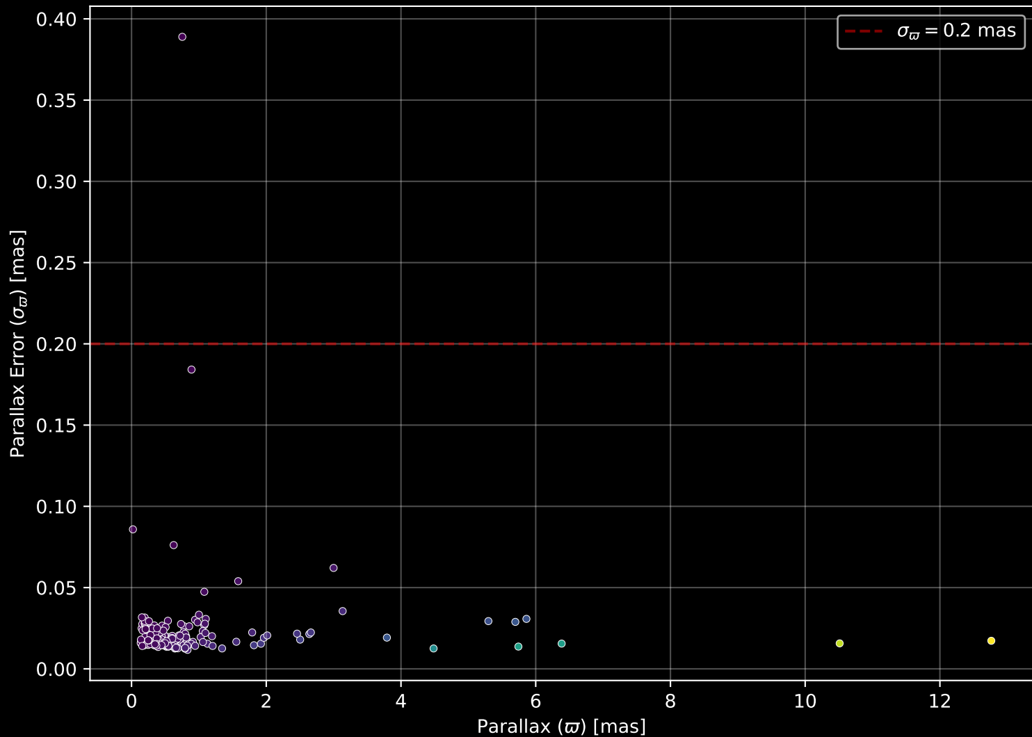
APOGEE DR17 Field: [150-08-RV] Parallax Quality (n= 191)
