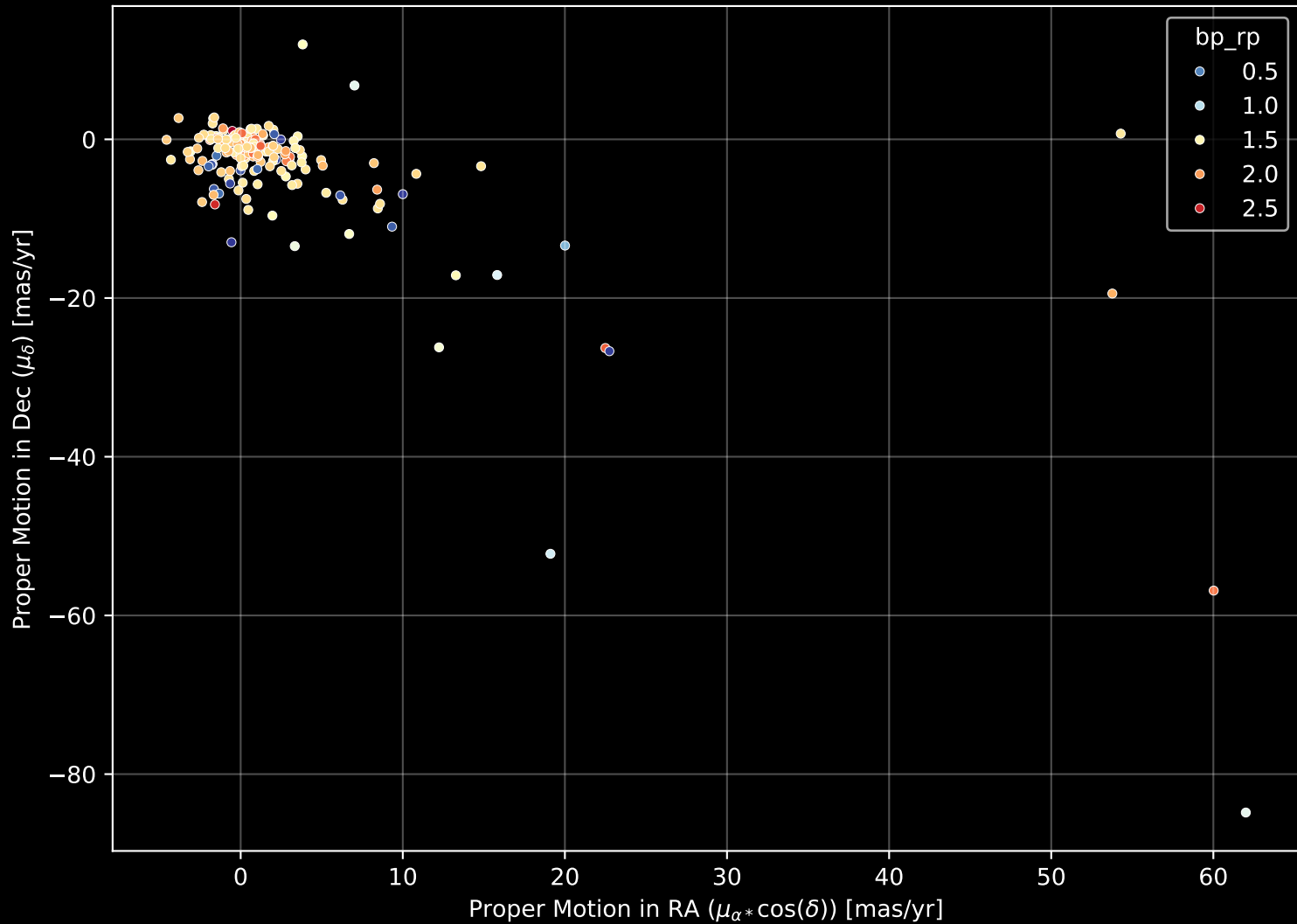
APOGEE DR17 Field: [150-08-RV] Proper Motion Diagram (n= 191)
