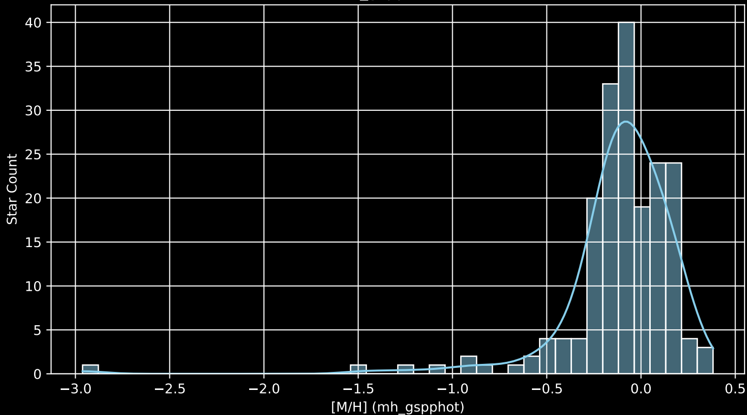
APOGEE DR17 Field: [150-08-RV [M/H] (mh_gspphot) (n= 189)
